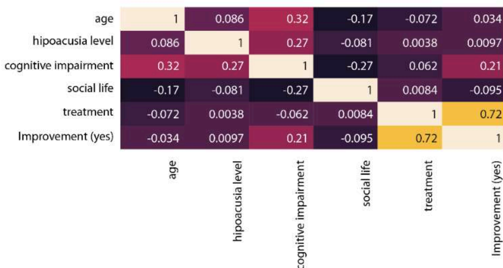
Figure 3: Correlation map
